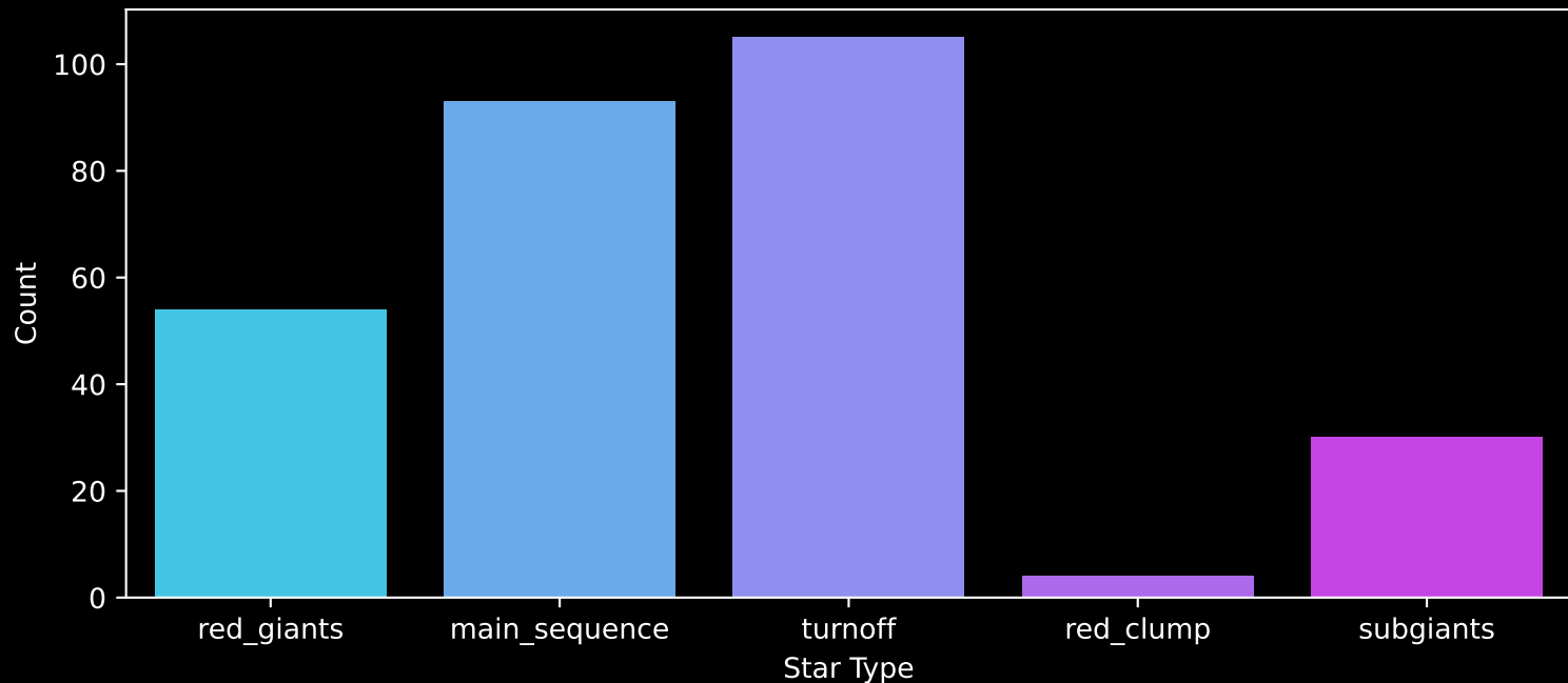
GALAH DR4 Field: [1552] Count plot of Star Type
