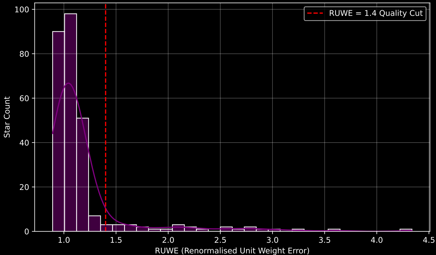
GALAH DR4 Field [1552] RUWE Distribution (n= 275)
